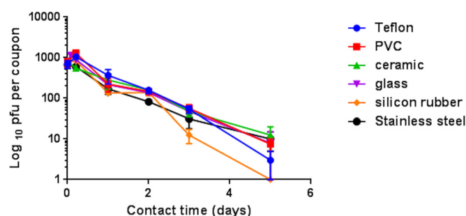
FIG 1 Persistence of infectious human coronavirus on common surface materials. Approximately 10^3 PFU HuCoV-229E (20 \mu l infected-cell lysate) was applied to 1-cm 2 coupons of test surface materials and incubated at ambient conditions (21°C; relative humidity, 30% to 40%). Virus was removed and assayed for infectivity at various time points as described in the text. Although the initial inoculum concentration was quite low, the virus retained infectivity for 5 days on all surfaces, except silicon rubber. Therefore, natural contamination of common surface material with very few coronavirus particles could represent a considerable risk of infection spread if touched and transferred to facial mucosa. Error bars represent \pm SEM, and data are from the results of multiple experiments.
